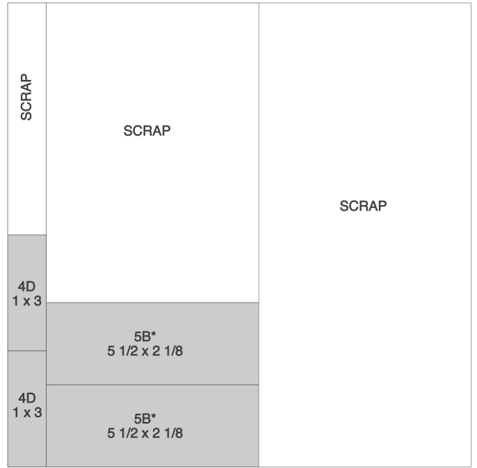
Cut Orientation
