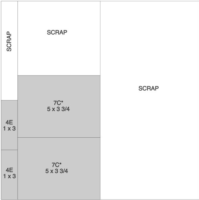
Cut Orientation
