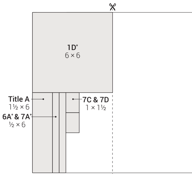
cut orientation
